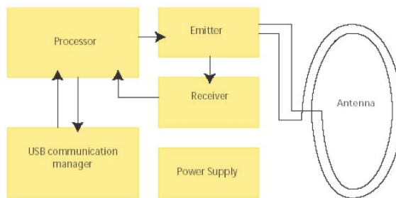
Functional scheme
