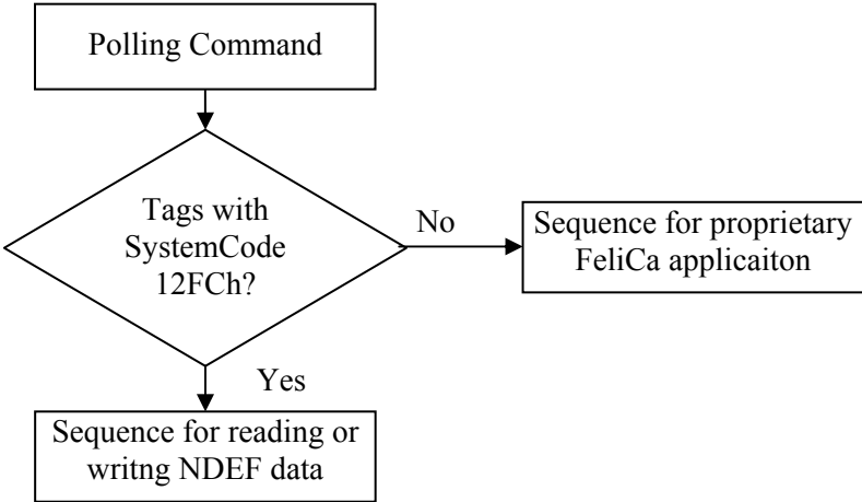
Figure 12: General sequence for detecting NDEF data
